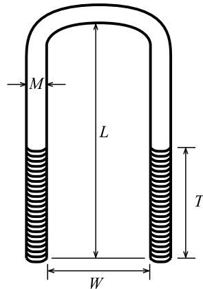
SEMI ROUND TOP FORM C
