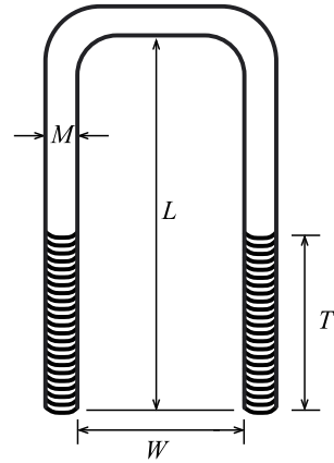
SQUARE TOP ROUND CORNER FORM B
