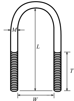
ROUND TOP FORM D
